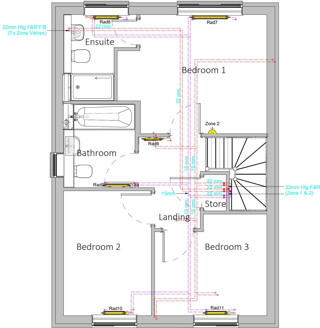
1 First Floor Heating GA 1 : 50
